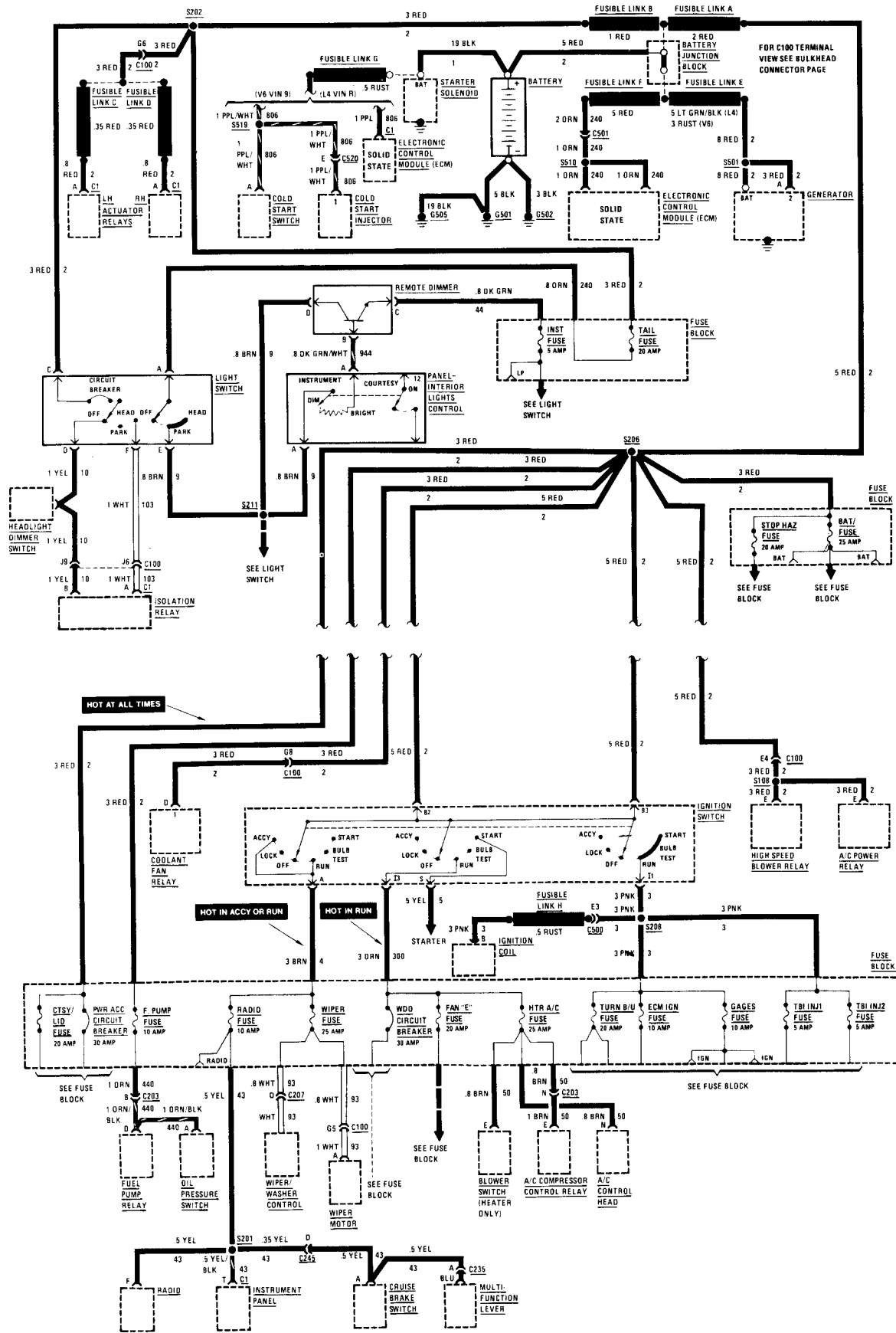
Power distribution
